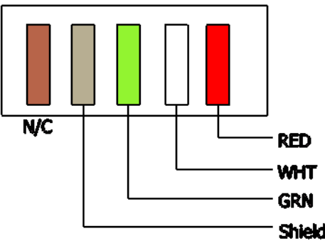
XBox 360 Cable (Controller End)
