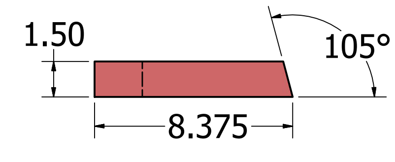
Upper Attachment (x3)
