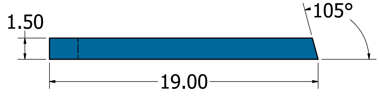
Lower Attachment (x3)
