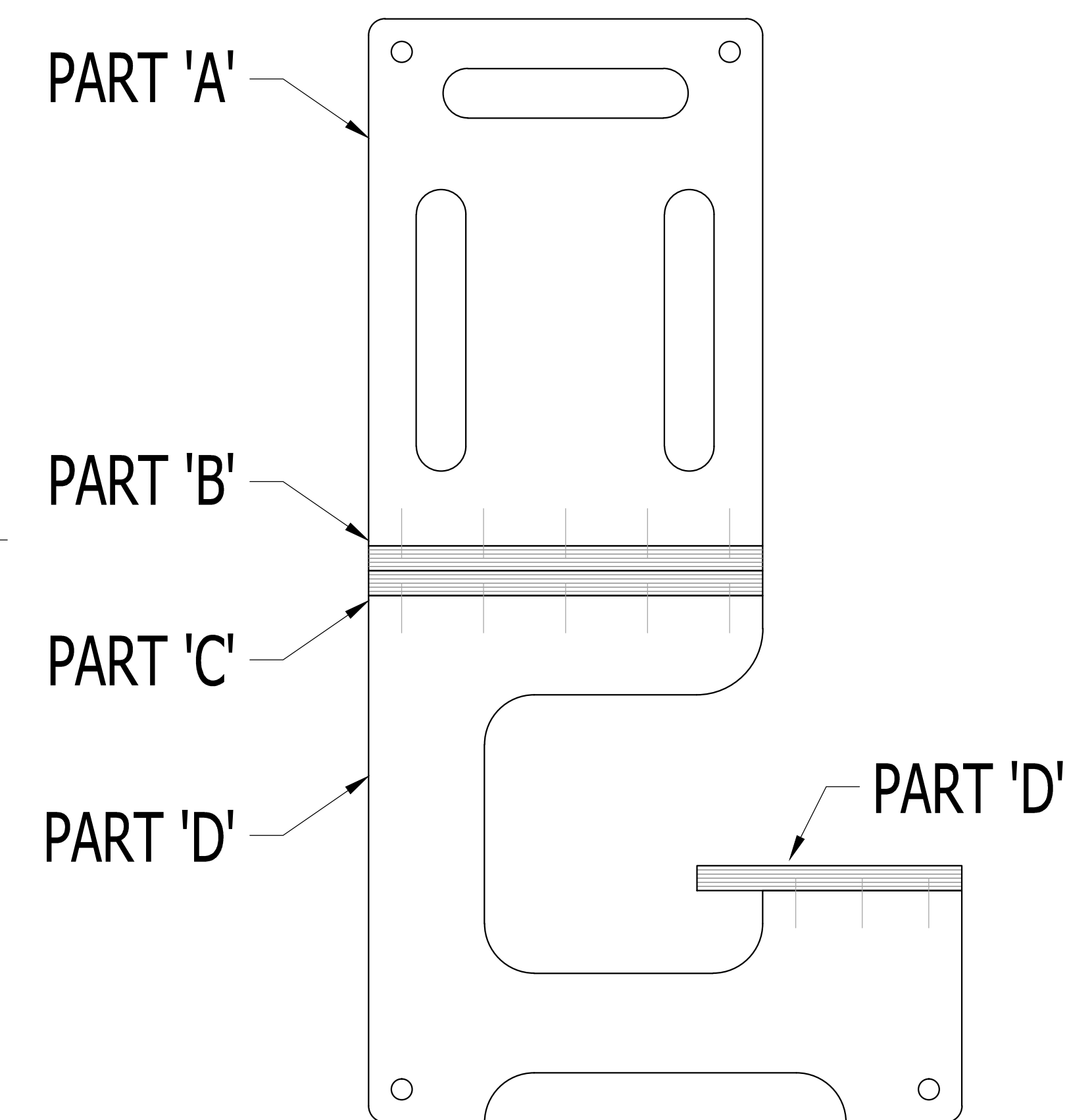
SIDE VIEW
