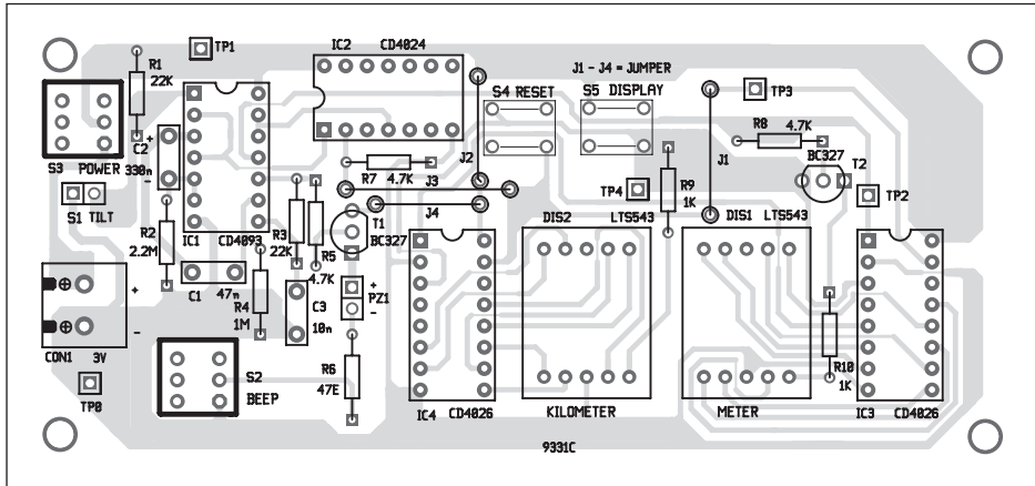
Fig. 4: Component layout for the PCB
