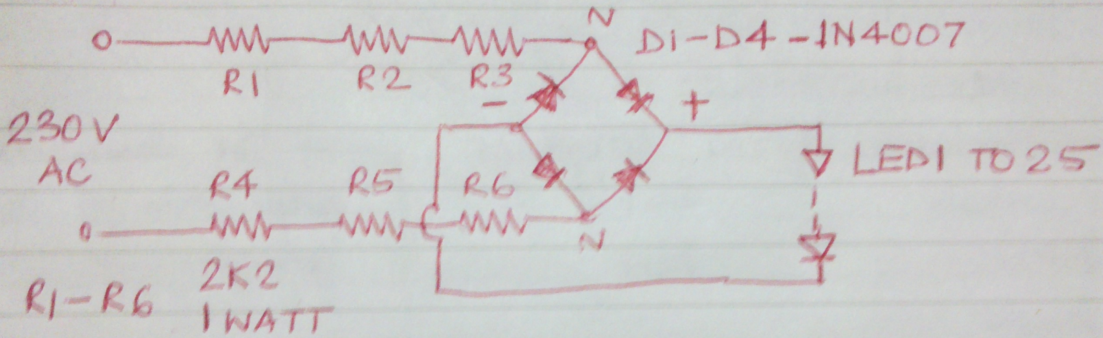
25 LED CIRCUIT DIAGRAM
